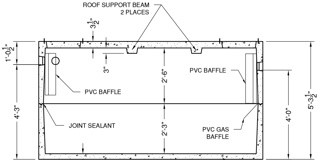
SECTION VIEW
